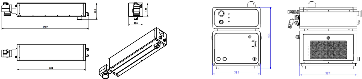
Dimensions (mm)
