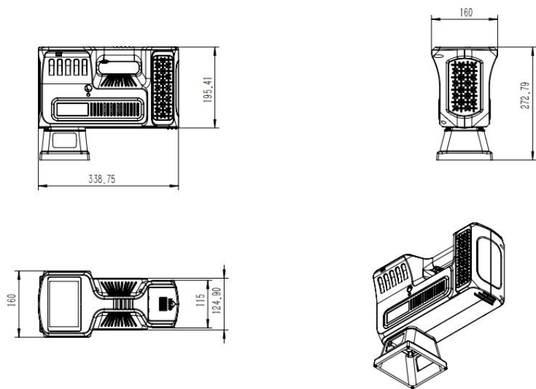
Dimensions (mm)
